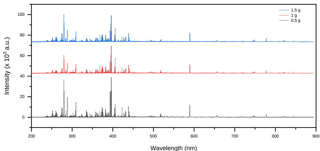
Figure 1. Complete LIBS spectra of bentonite containing Pb.
